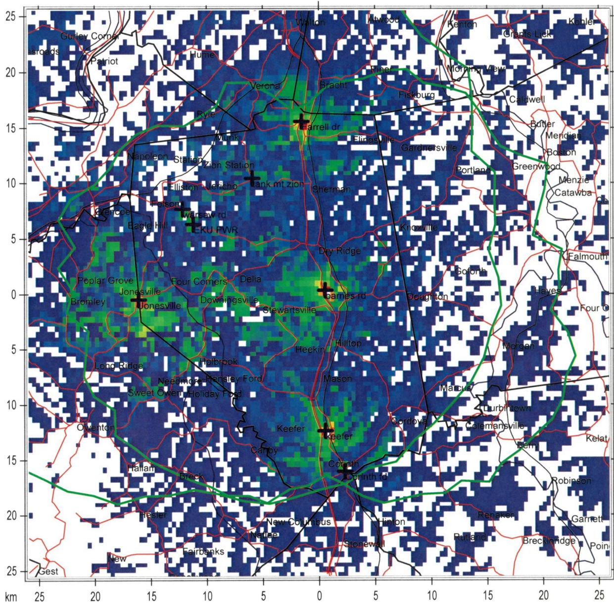
System Composite Talk Back
